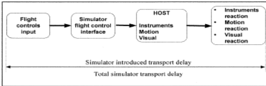
Figure A2C Transport Delay for simulation of classic non-computer controlled aircraft.
